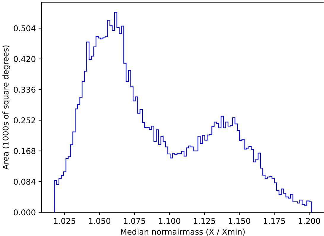
ddf_half_v3.4_10yrs All sky y band: Median normairmass
