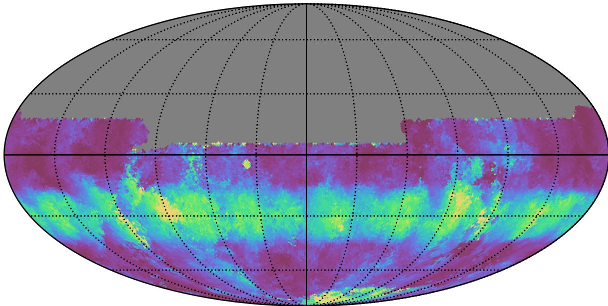
ddf_half_v3.4_10yrs All sky u band: Median normairmass
