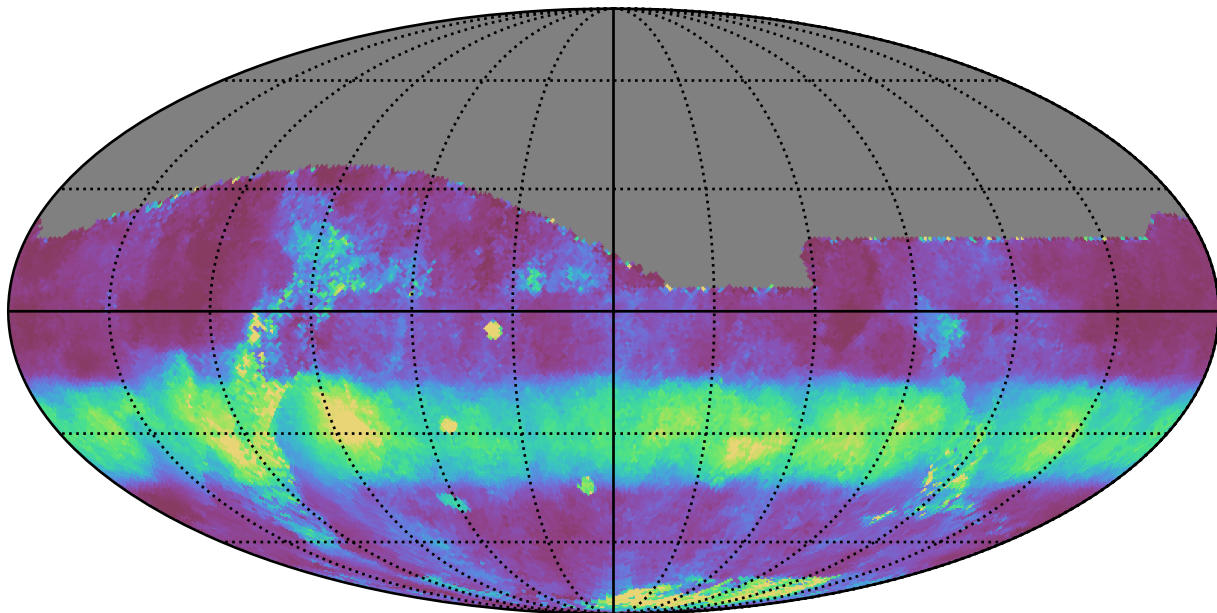
ddf_half_v3.4_10yrs All sky r band: Median normairmass
