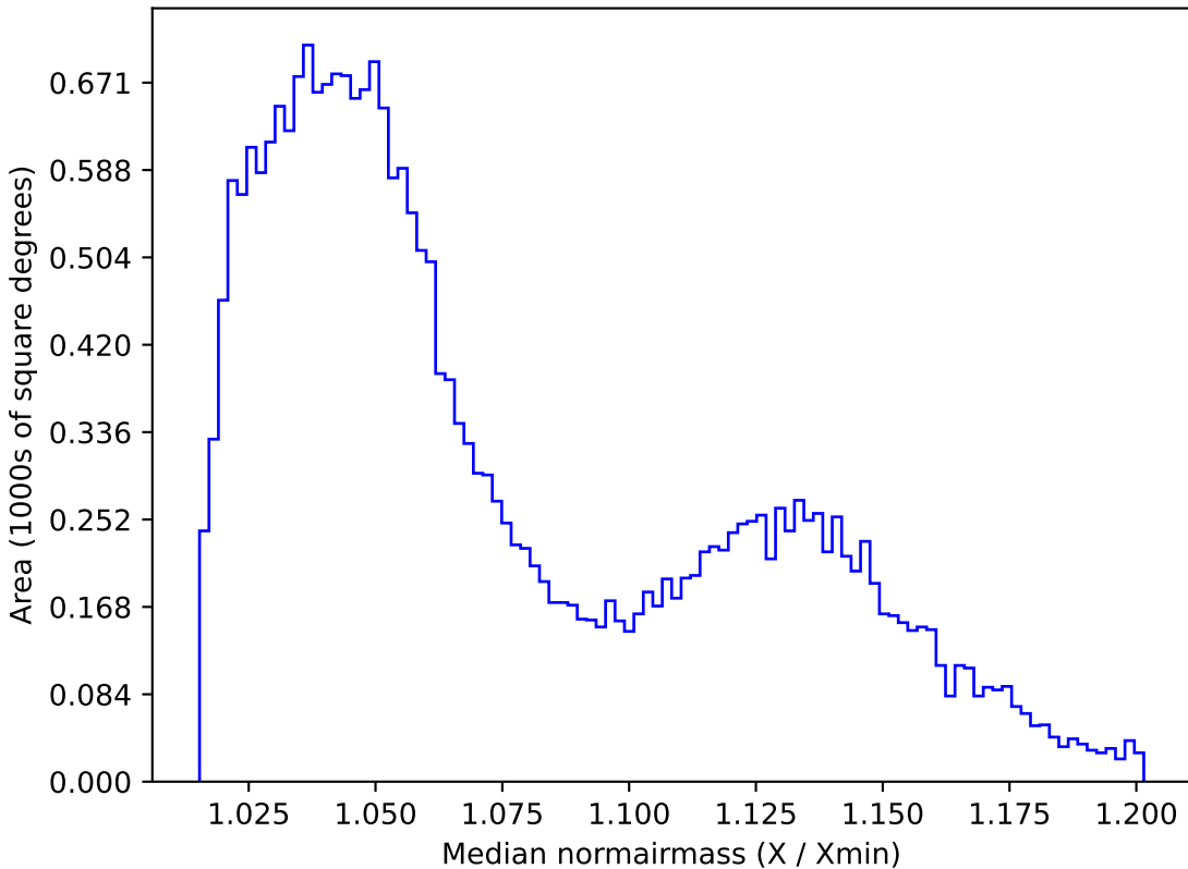
ddf_half_v3.4_10yrs All sky r band: Median normairmass
