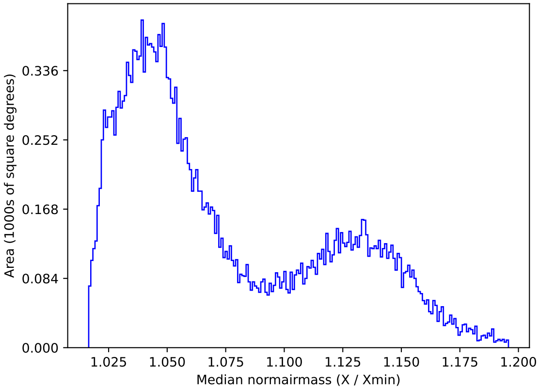
ddf_half_v3.4_10yrs All sky i band: Median normairmass
