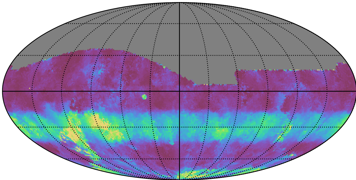
ddf_half_v3.4_10yrs All sky g band: Median normairmass
