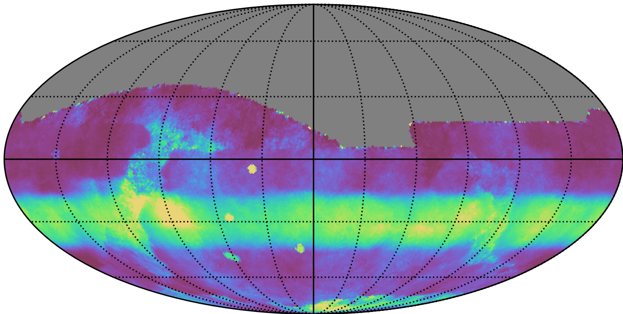
ddf_half_v3.4_10yrs All sky all bands: Median normairmass
