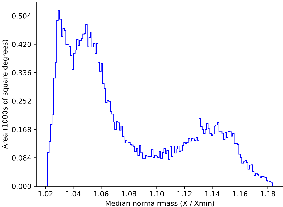
ddf_half_v3.4_10yrs All sky all bands: Median normairmass
