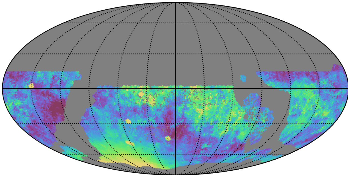
ddf_half_v3.4_10yrs WFD z band: Median moonDistance
