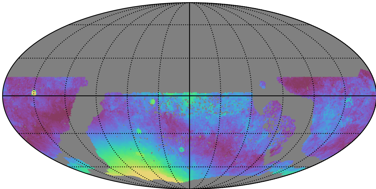
ddf_half_v3.4_10yrs WFD y band: Median moonDistance
