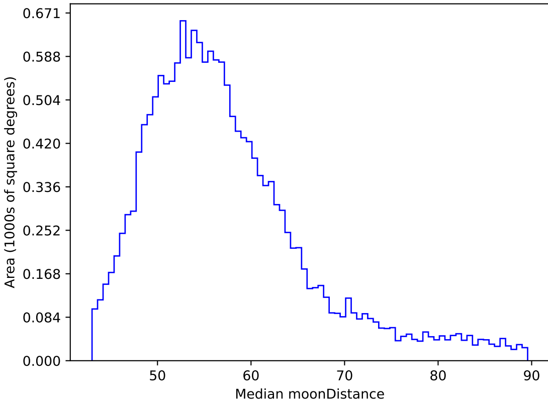
ddf_half_v3.4_10yrs WFD y band: Median moonDistance
