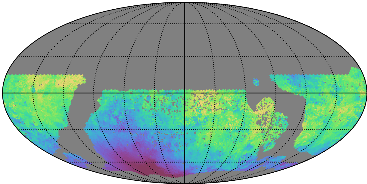
ddf_half_v3.4_10yrs WFD u band: Median moonDistance
