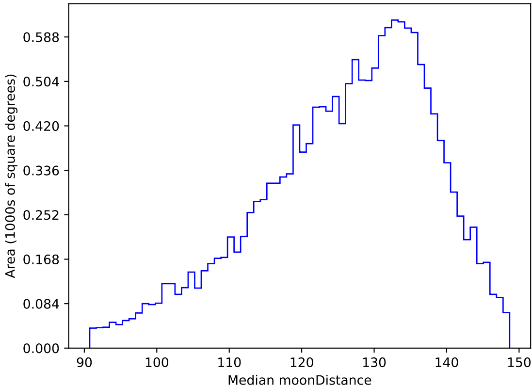
ddf_half_v3.4_10yrs WFD u band: Median moonDistance
