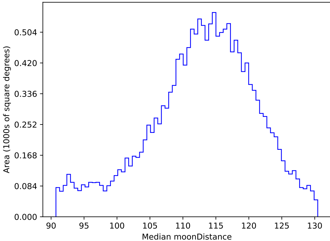
ddf_half_v3.4_10yrs WFD r band: Median moonDistance
