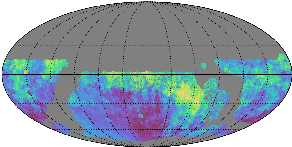
ddf_half_v3.4_10yrs WFD i band: Median moonDistance
