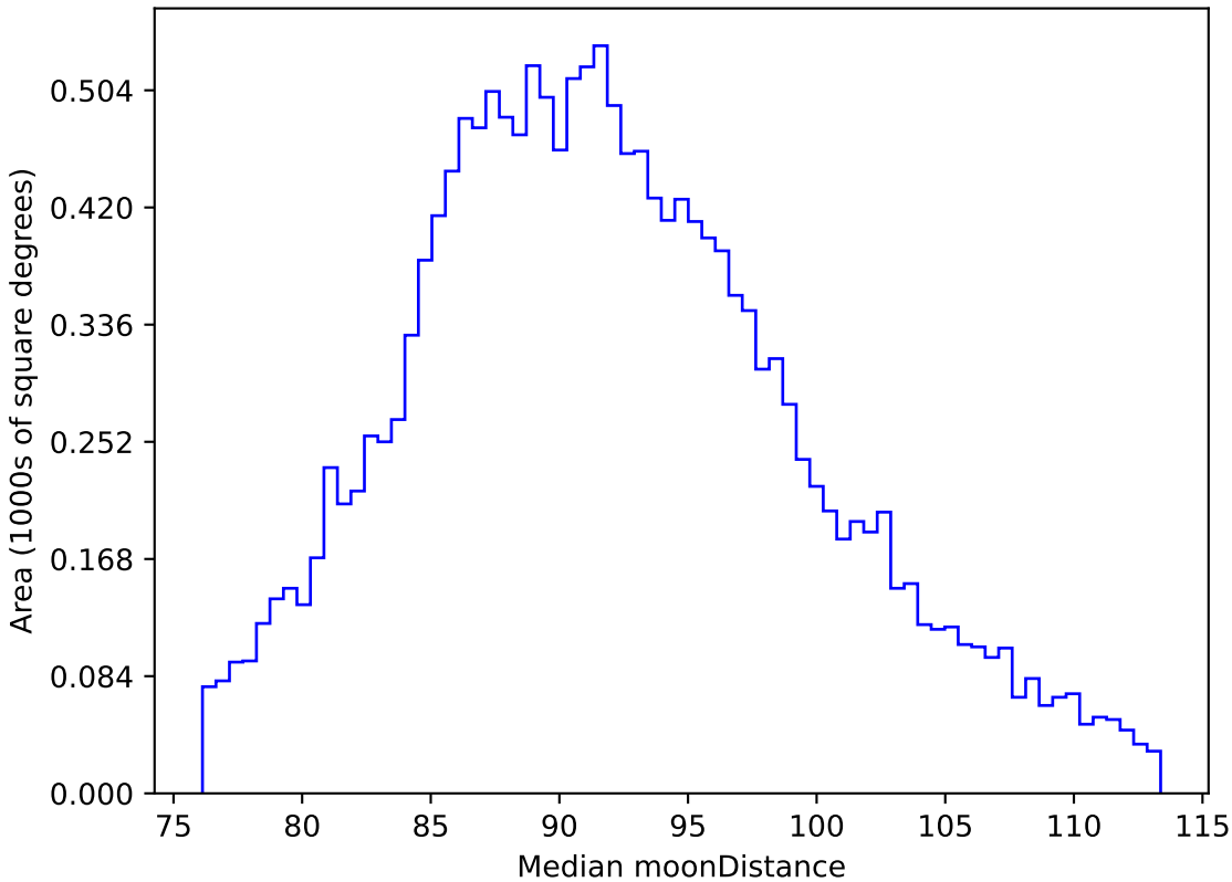
ddf_half_v3.4_10yrs WFD i band: Median moonDistance
