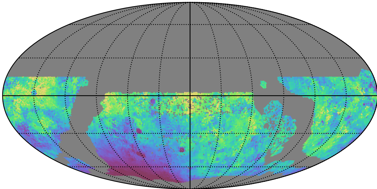
ddf_half_v3.4_10yrs WFD g band: Median moonDistance
