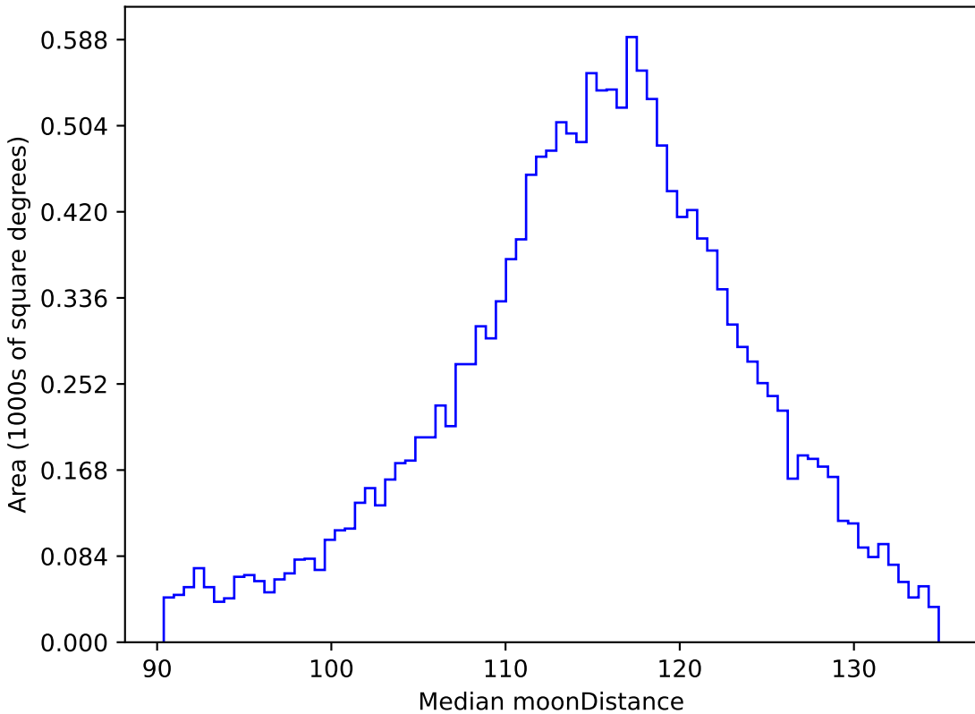
ddf_half_v3.4_10yrs WFD g band: Median moonDistance
