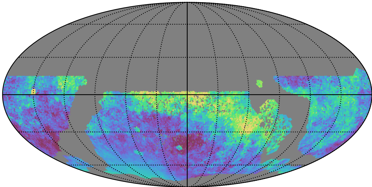
ddf_half_v3.4_10yrs WFD all bands: Median moonDistance
