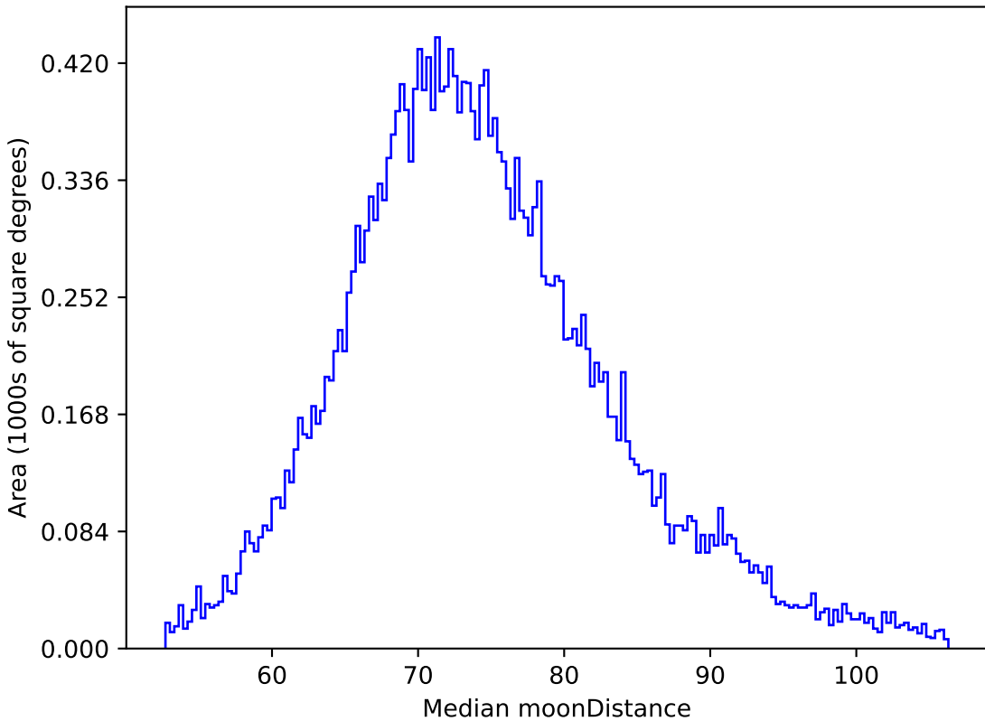
ddf_half_v3.4_10yrs All sky z band: Median moonDistance
