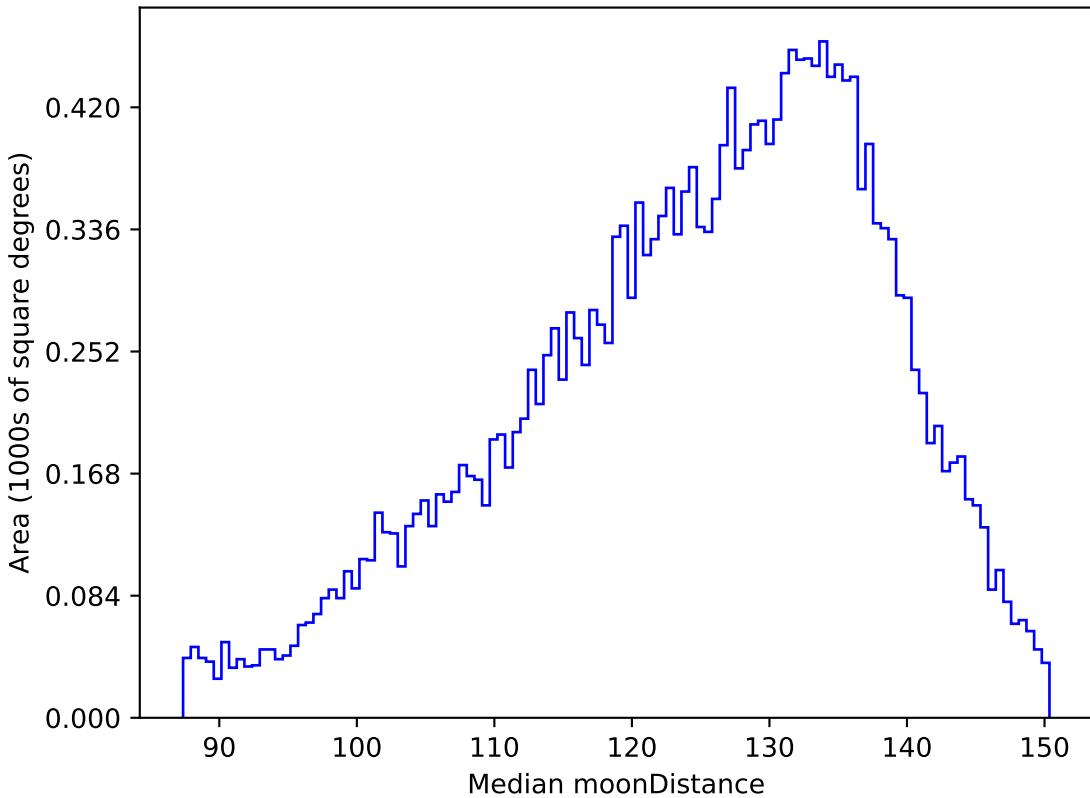
ddf_half_v3.4_10yrs All sky u band: Median moonDistance
