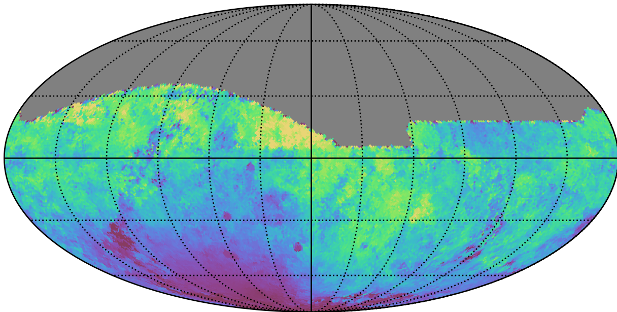
ddf_half_v3.4_10yrs All sky r band: Median moonDistance
