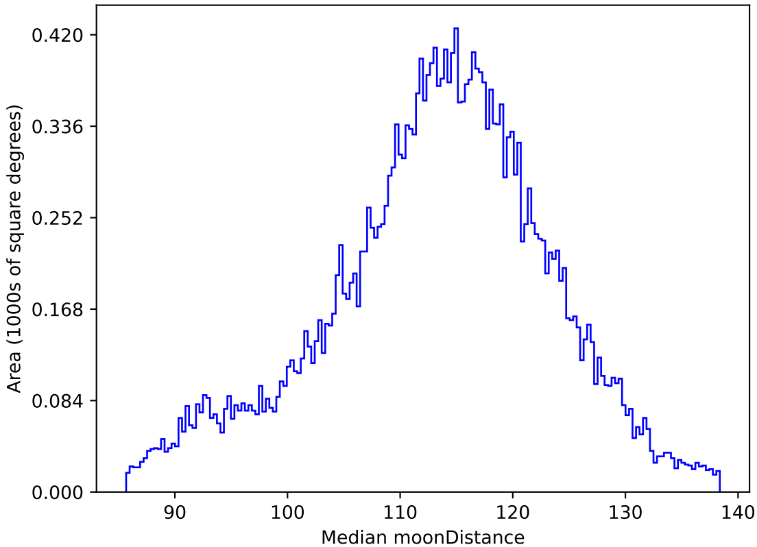
ddf_half_v3.4_10yrs All sky r band: Median moonDistance
