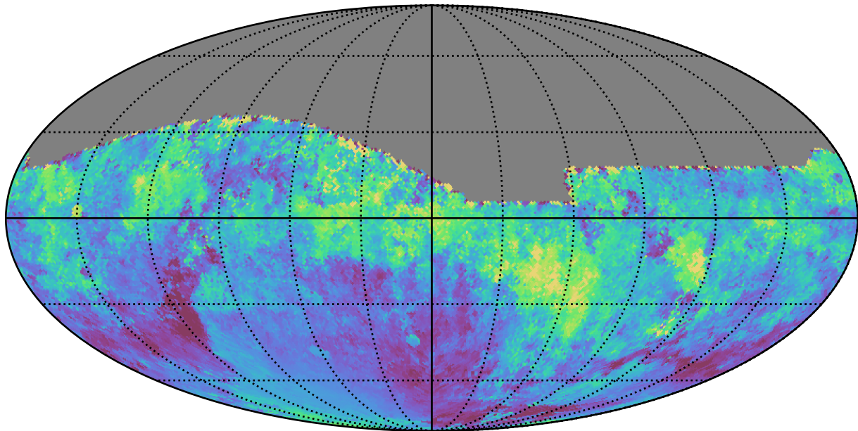
ddf_half_v3.4_10yrs All sky i band: Median moonDistance
