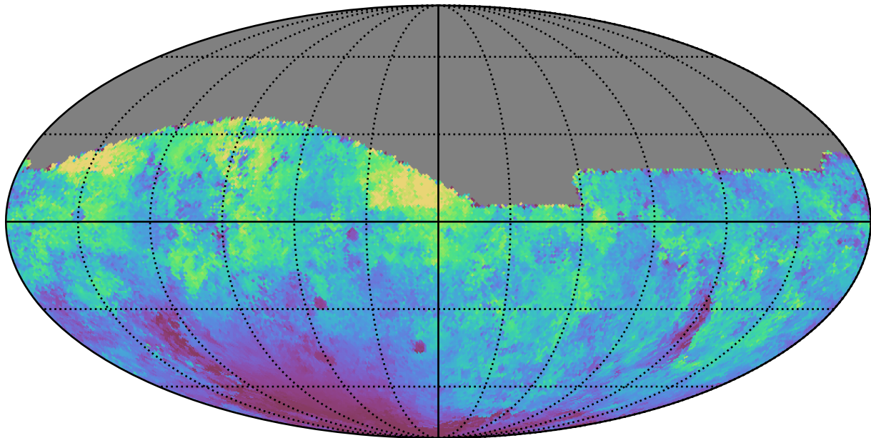
ddf_half_v3.4_10yrs All sky g band: Median moonDistance
