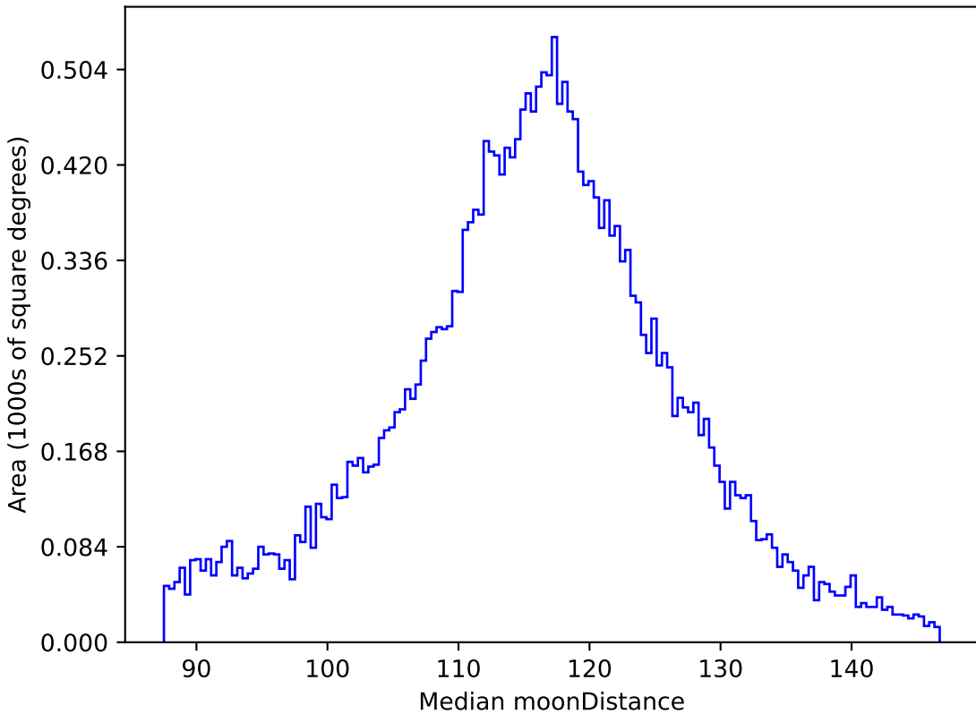
ddf_half_v3.4_10yrs All sky g band: Median moonDistance
