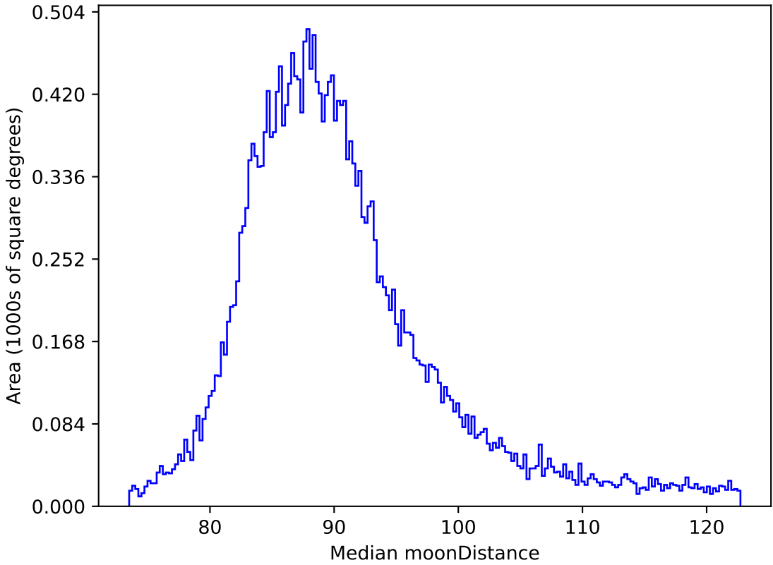
ddf_half_v3.4_10yrs All sky all bands: Median moonDistance
