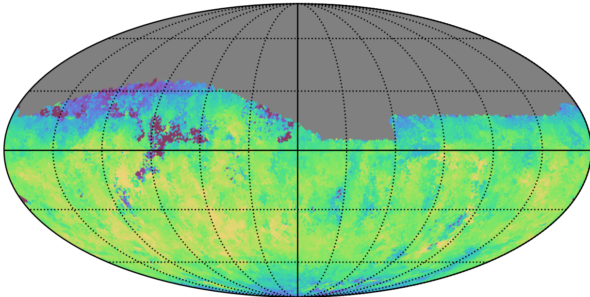
ddf_half_v3.4_10yrs Yr 1 z band: Median fiveSigmaDepth
