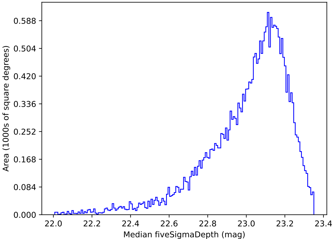
ddf_half_v3.4_10yrs Yr 1 z band: Median fiveSigmaDepth
