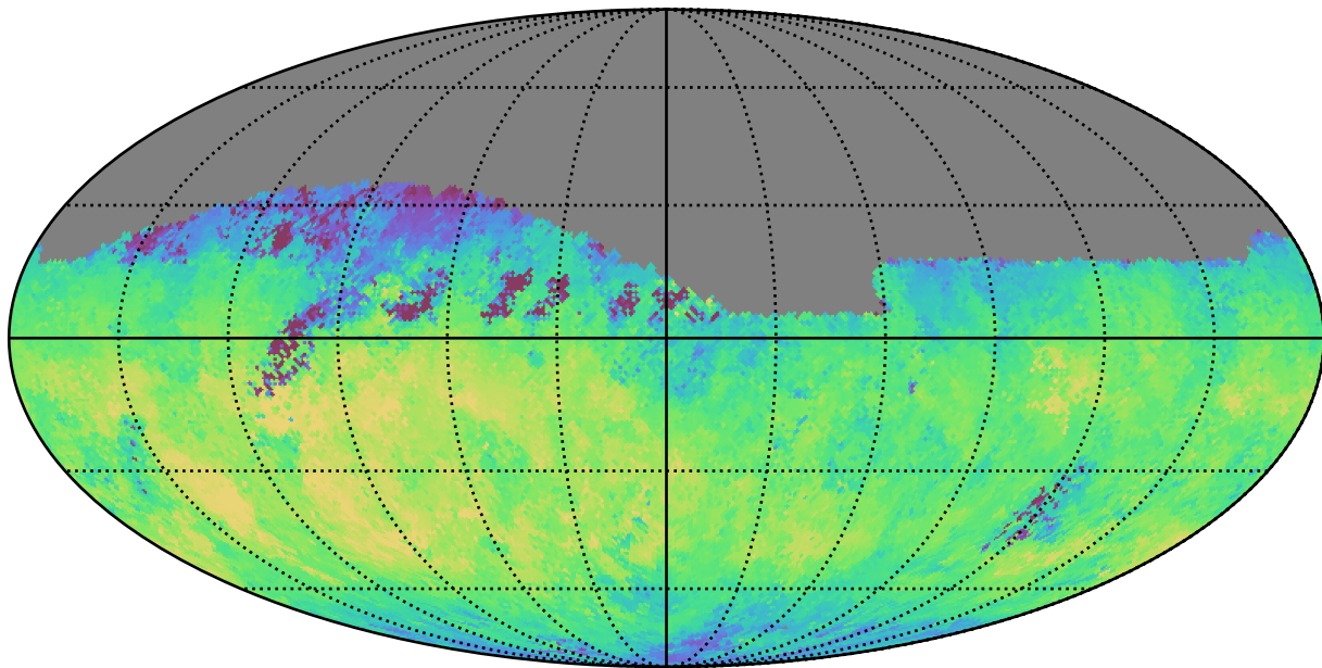
ddf_half_v3.4_10yrs Yr 1 r band: Median fiveSigmaDepth
