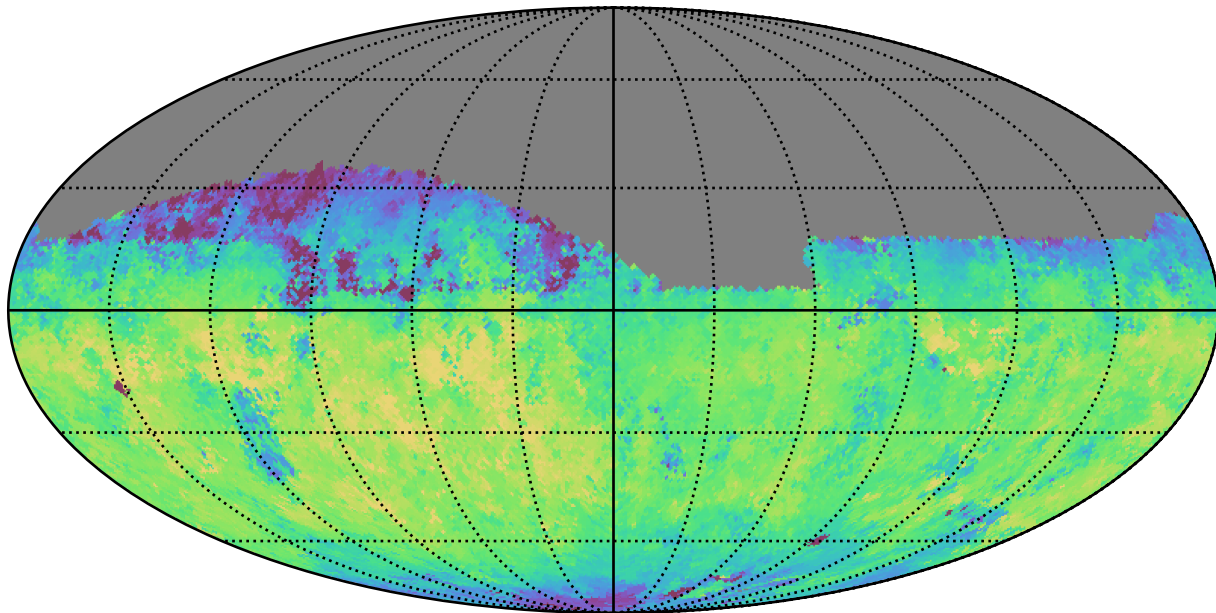
ddf_half_v3.4_10yrs Yr 1 i band: Median fiveSigmaDepth
