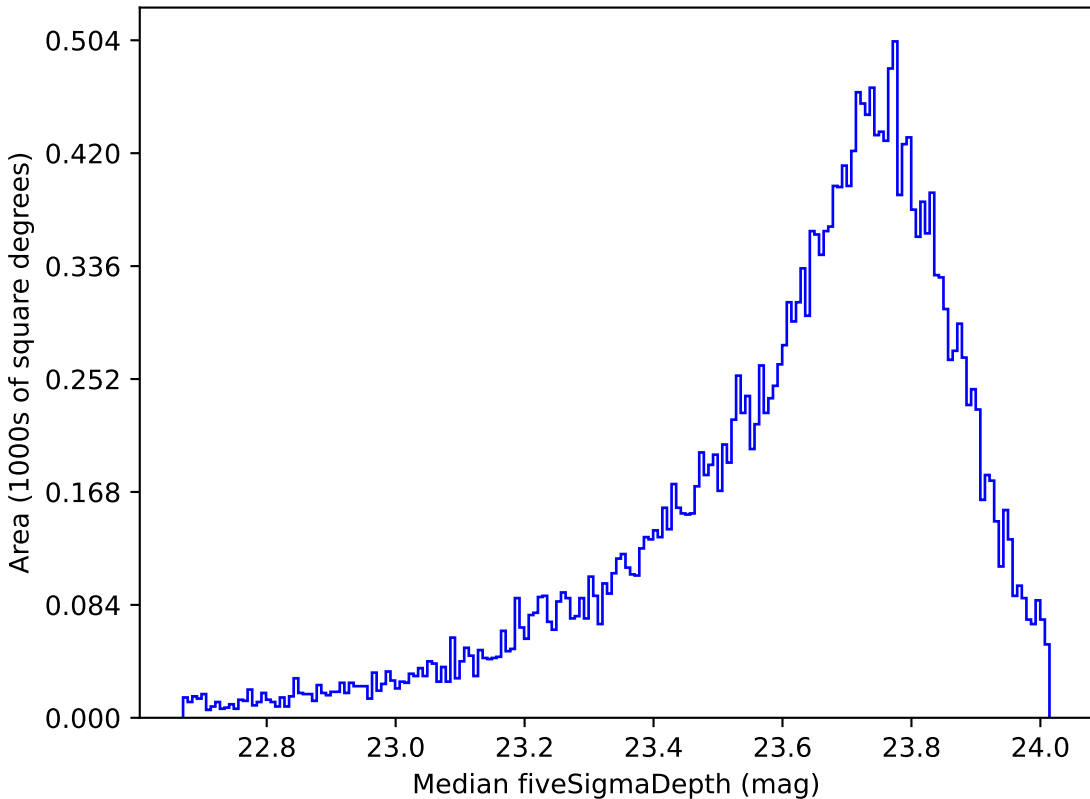
ddf_half_v3.4_10yrs Yr 1 i band: Median fiveSigmaDepth
