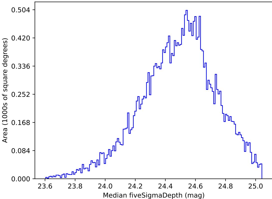
ddf_half_v3.4_10yrs Yr 1 g band: Median fiveSigmaDepth
