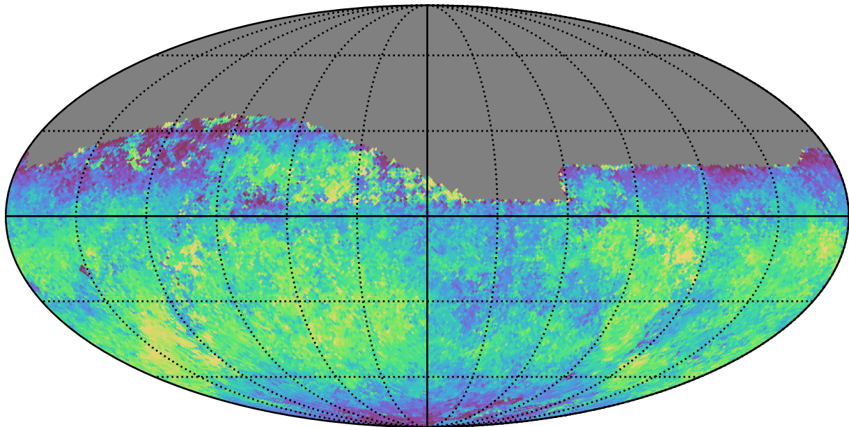
ddf_half_v3.4_10yrs Yr 1 all bands: Median fiveSigmaDepth
