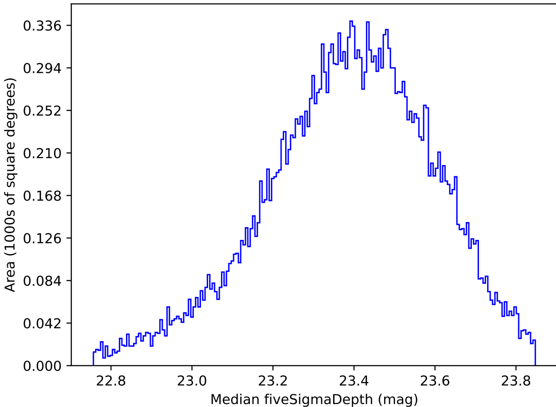
ddf_half_v3.4_10yrs Yr 1 all bands: Median fiveSigmaDepth
