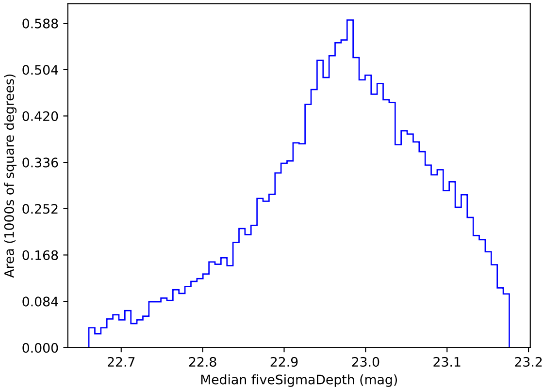
ddf_half_v3.4_10yrs WFD z band: Median fiveSigmaDepth
