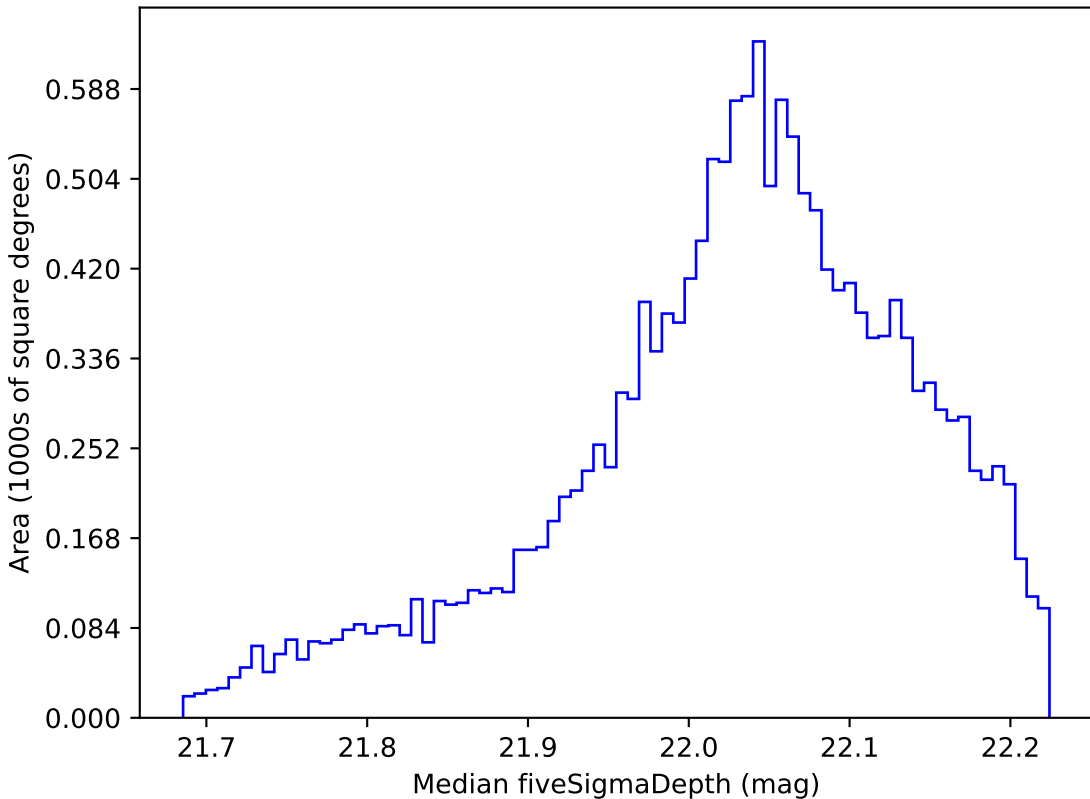
ddf_half_v3.4_10yrs WFD y band: Median fiveSigmaDepth
