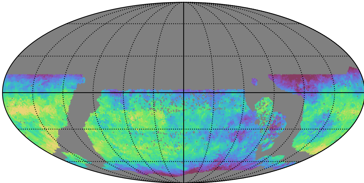
ddf_half_v3.4_10yrs WFD u band: Median fiveSigmaDepth
