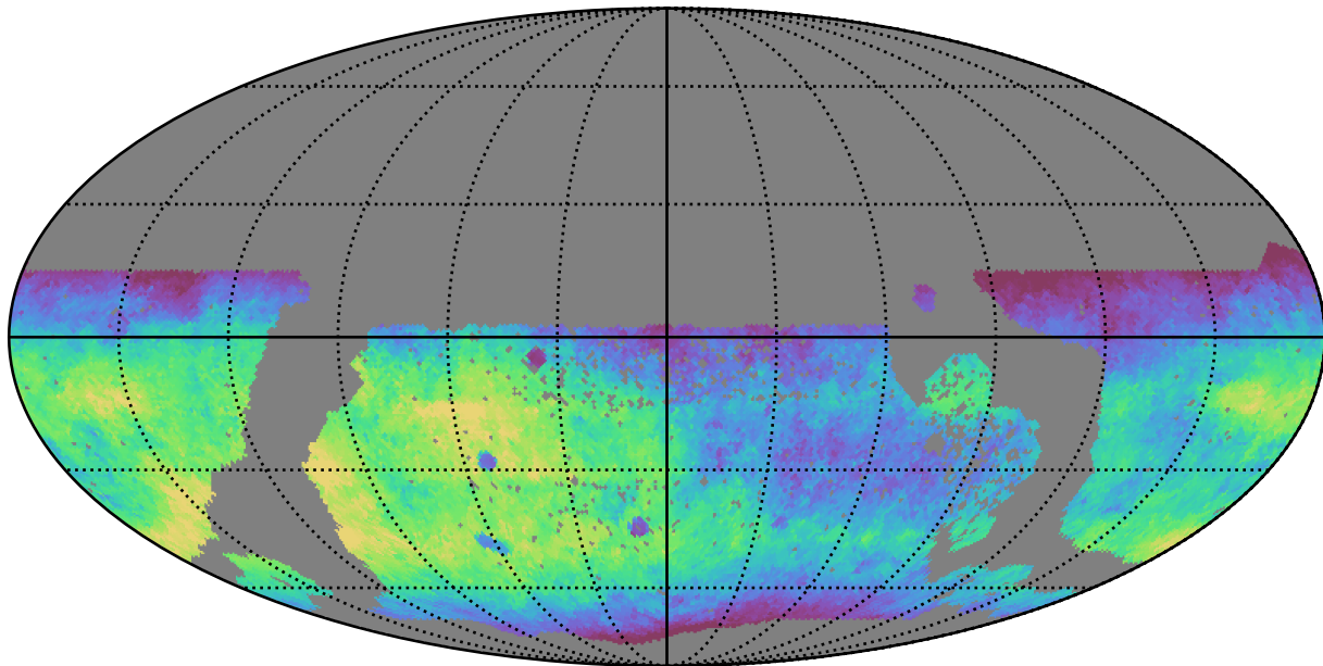
ddf_half_v3.4_10yrs WFD r band: Median fiveSigmaDepth
