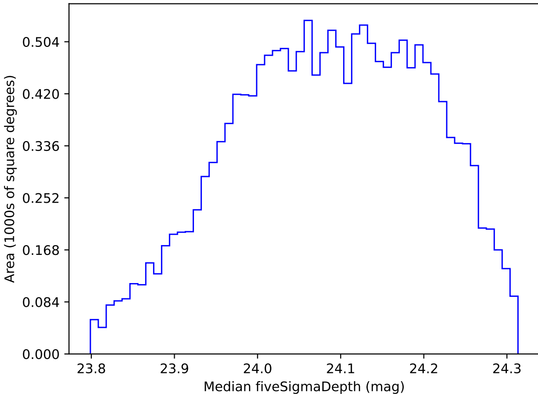
ddf_half_v3.4_10yrs WFD r band: Median fiveSigmaDepth
