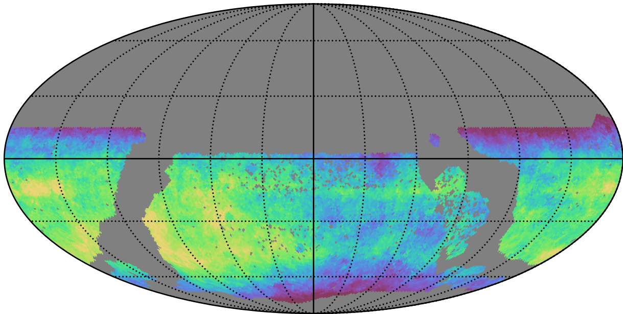
ddf_half_v3.4_10yrs WFD i band: Median fiveSigmaDepth
