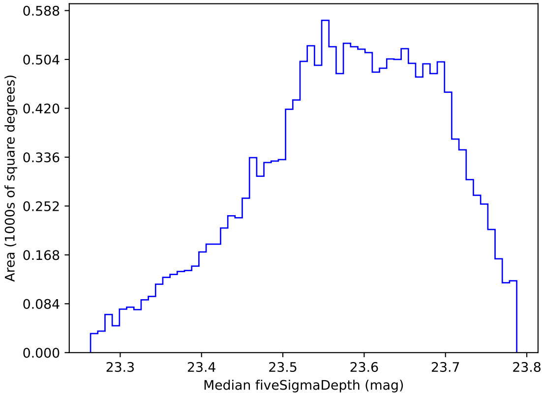
ddf_half_v3.4_10yrs WFD i band: Median fiveSigmaDepth
