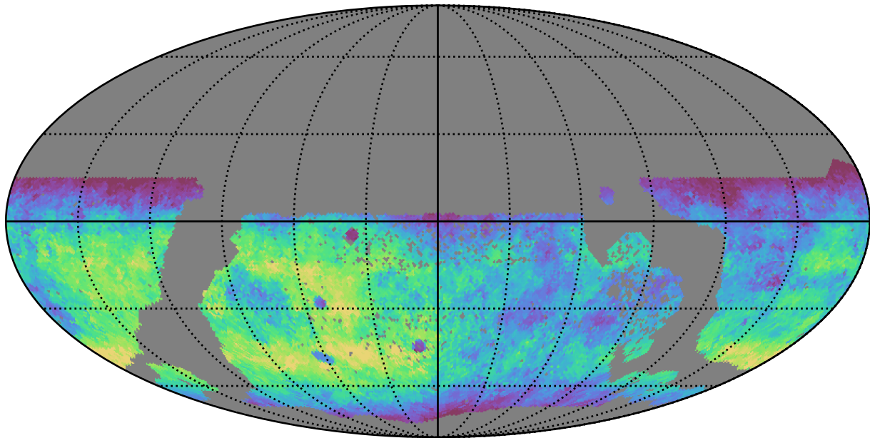
ddf_half_v3.4_10yrs WFD g band: Median fiveSigmaDepth
