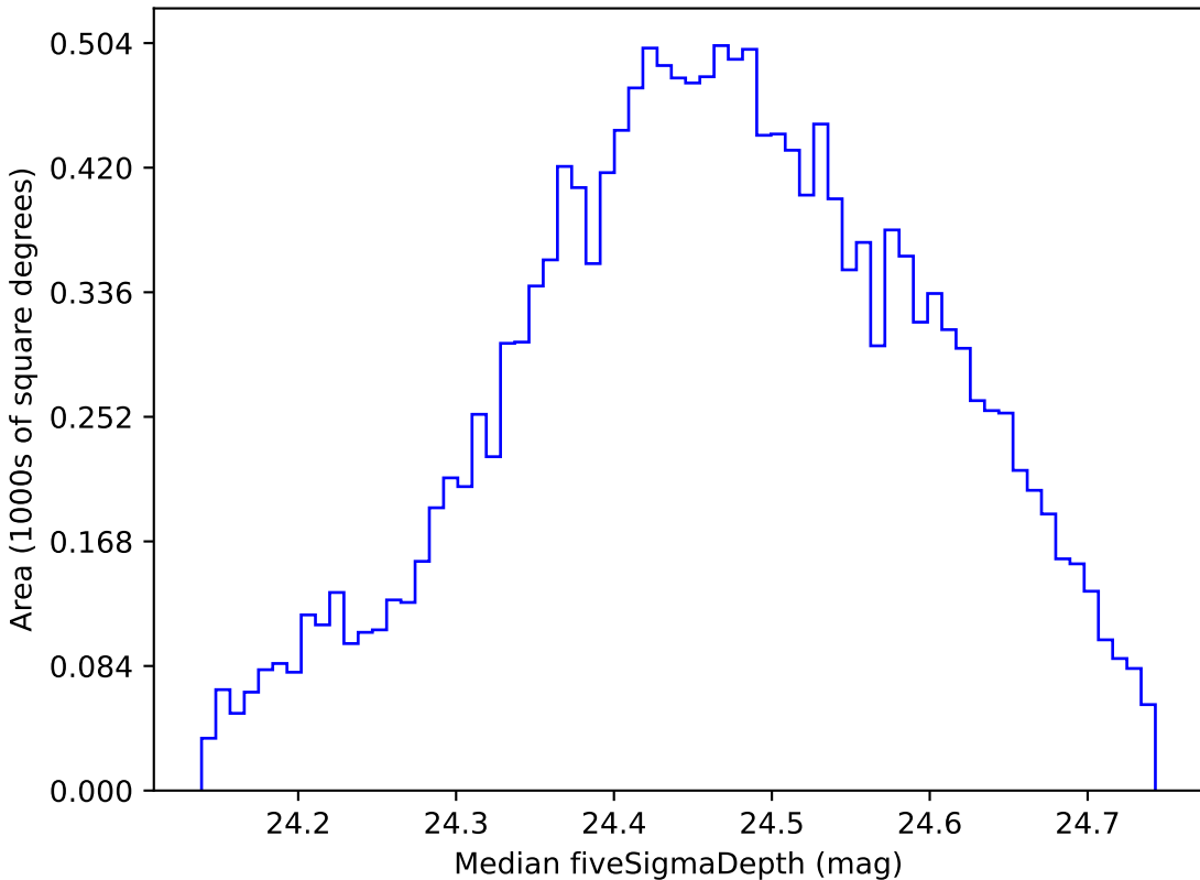
ddf_half_v3.4_10yrs WFD g band: Median fiveSigmaDepth
