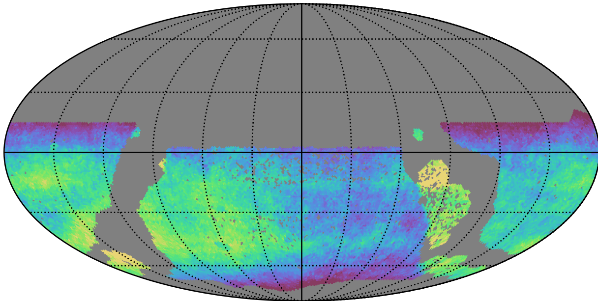
ddf_half_v3.4_10yrs WFD all bands: Median fiveSigmaDepth
