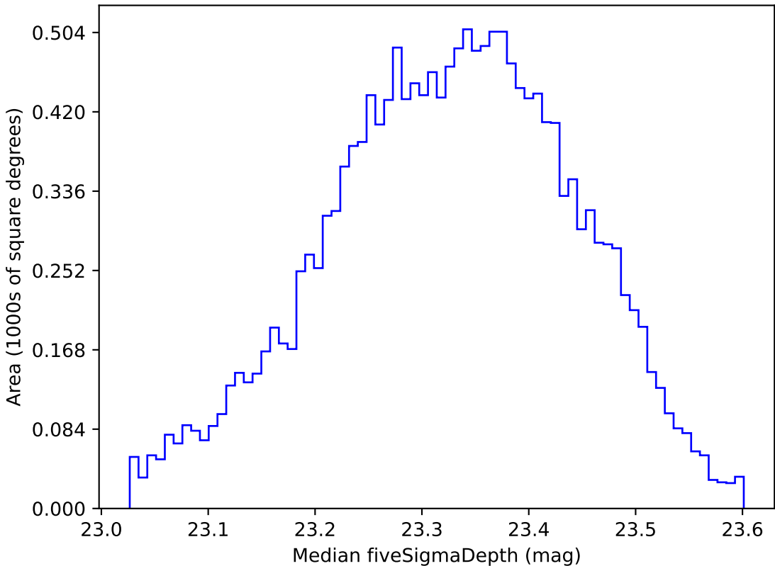
ddf_half_v3.4_10yrs WFD all bands: Median fiveSigmaDepth
