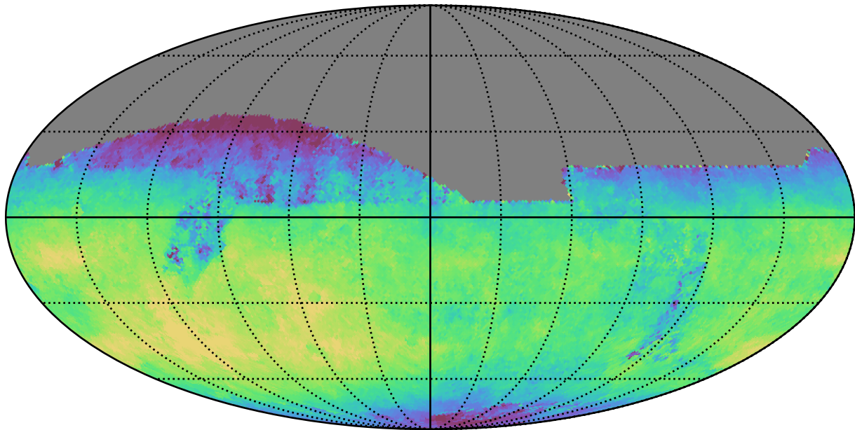
ddf_half_v3.4_10yrs All sky z band: Median fiveSigmaDepth
