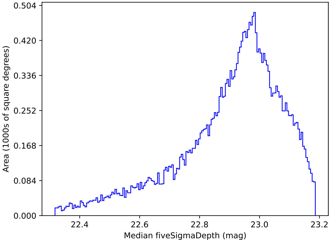
ddf_half_v3.4_10yrs All sky z band: Median fiveSigmaDepth
