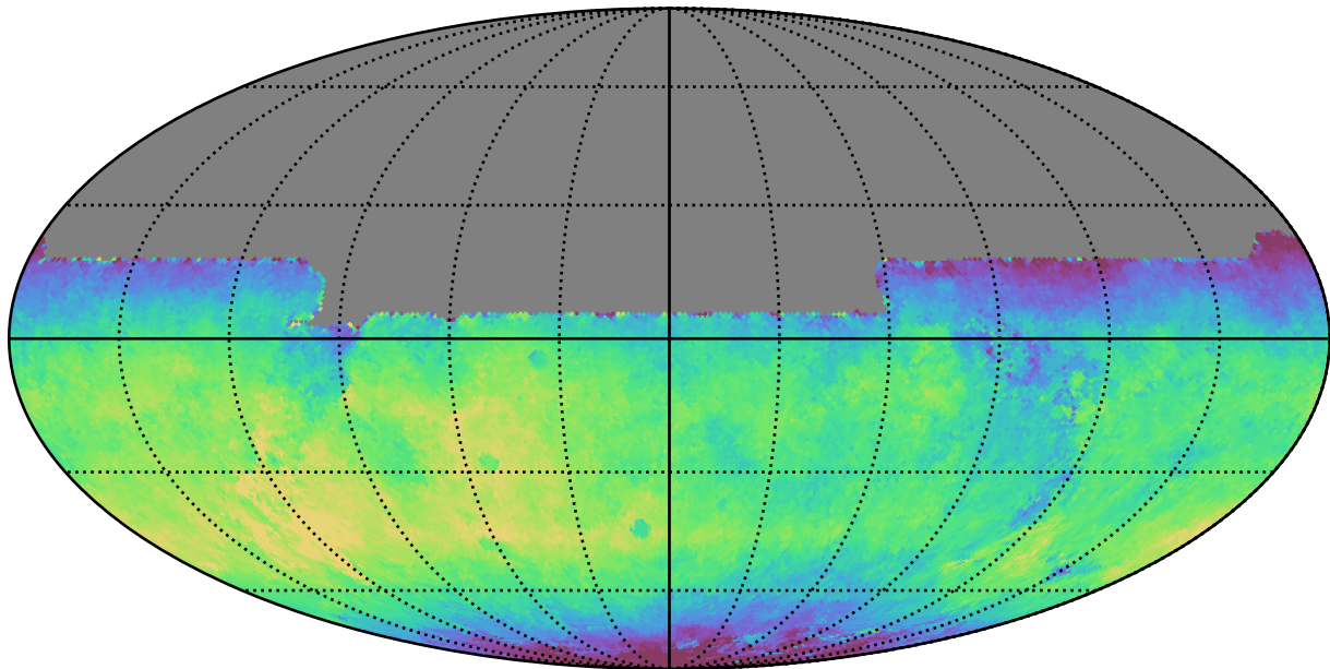
ddf_half_v3.4_10yrs All sky y band: Median fiveSigmaDepth
