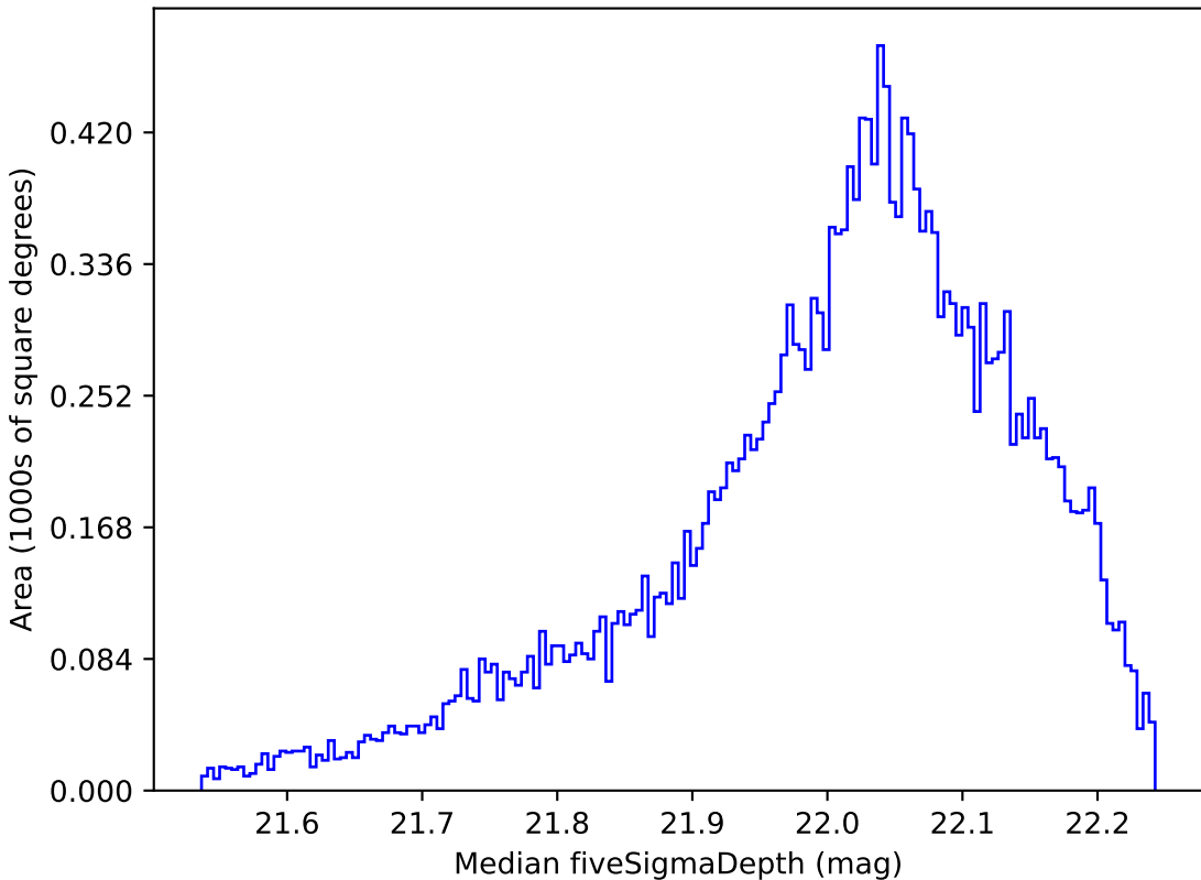
ddf_half_v3.4_10yrs All sky y band: Median fiveSigmaDepth
